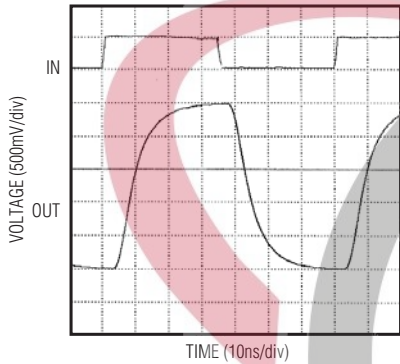
MAX4144 LARGE-SIGNAL PULSE RESPONSE ( A_V = +2 )
